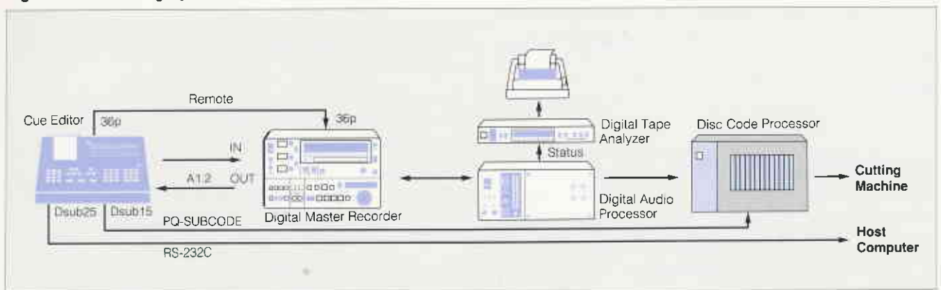
Fig. 27 CD Mastering System
