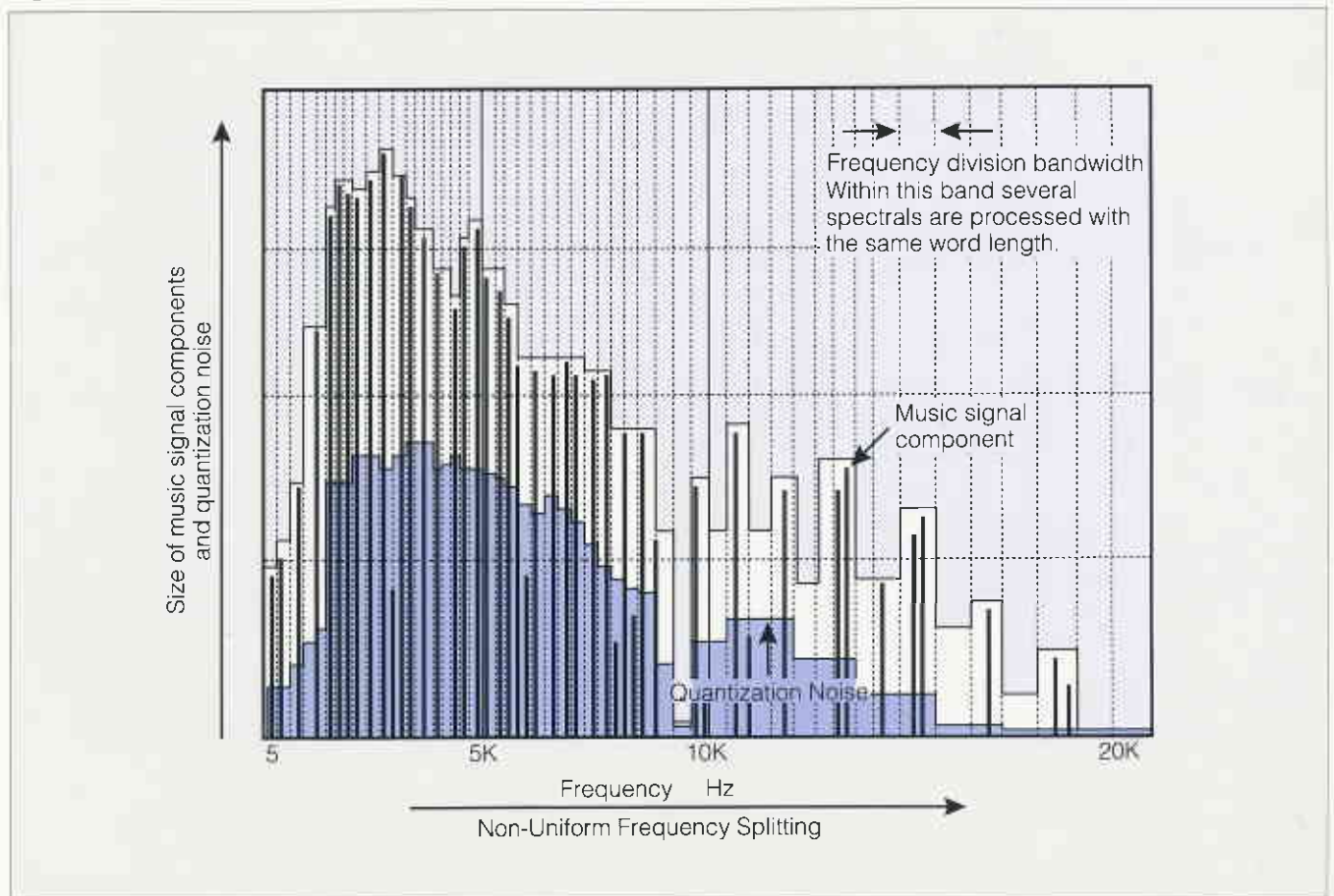
Fig. 16 ATRAC Effective Bit Allocation
