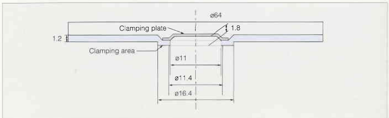
Fig.12 Cross-section of Disc and Clamping Plate
