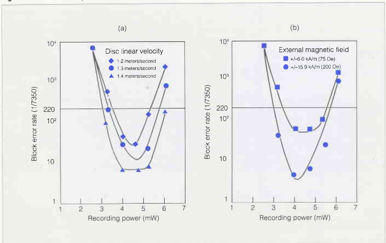
Fig. 24 Block Error Rate By Variations in Recording Power
