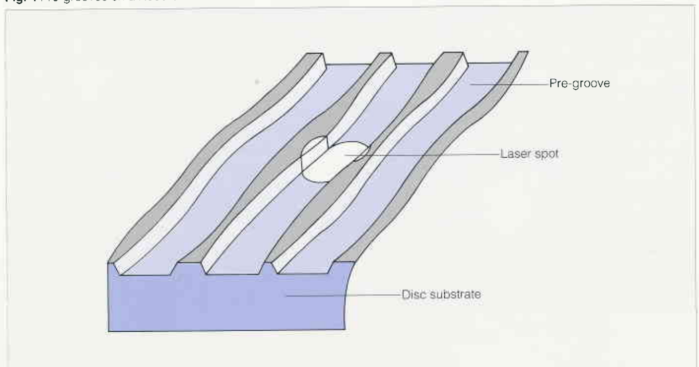
Fig. 4 Pre-grooves on a Recordable MiniDisc
