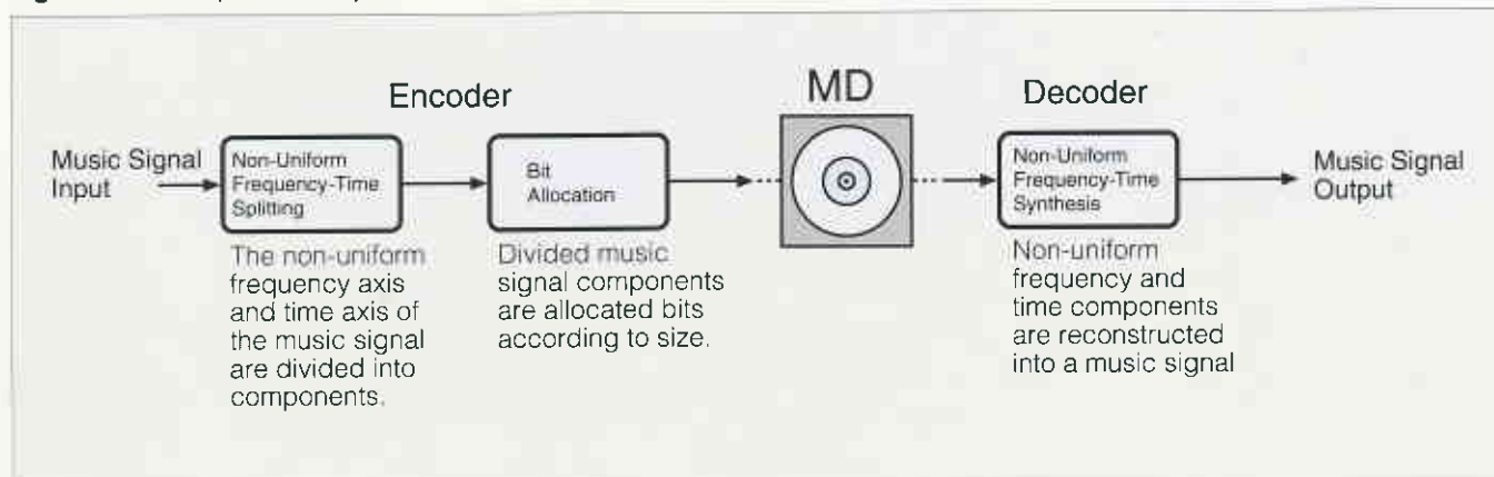
Fig. 15 ATRAC Operation Layout
