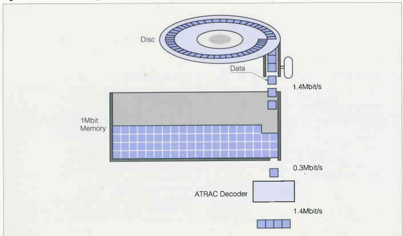
Fig. 1 Shock-resistant Memory
