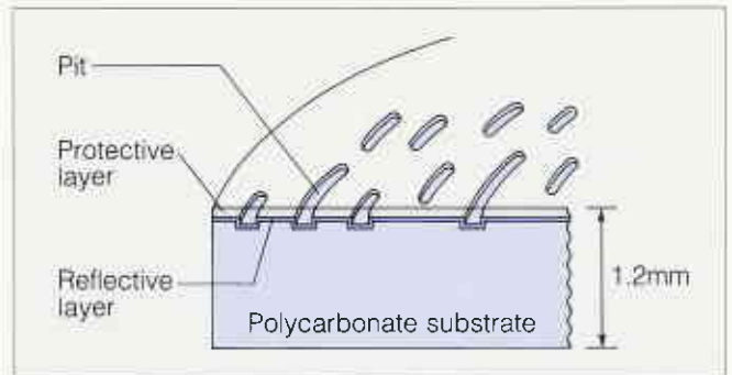
Fig. 8 Cross-sectional Representation of Disc Substrate
