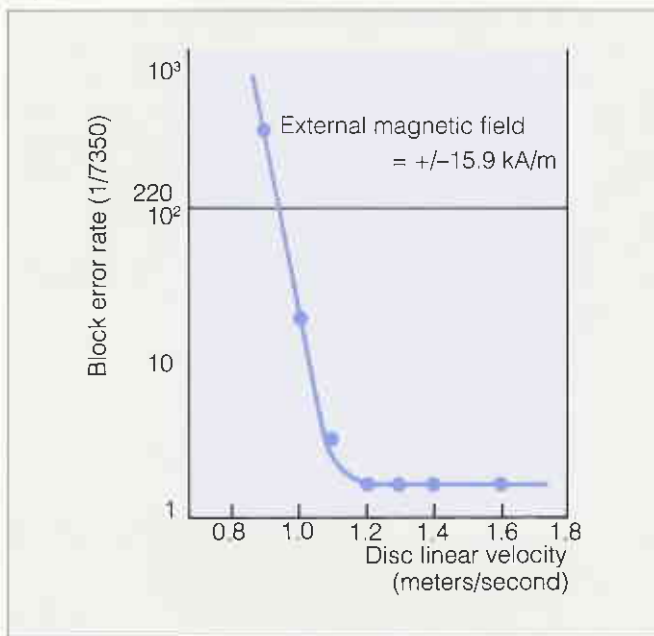
Fig. 22 Block Error Rate with Magnetic Field Modulation
