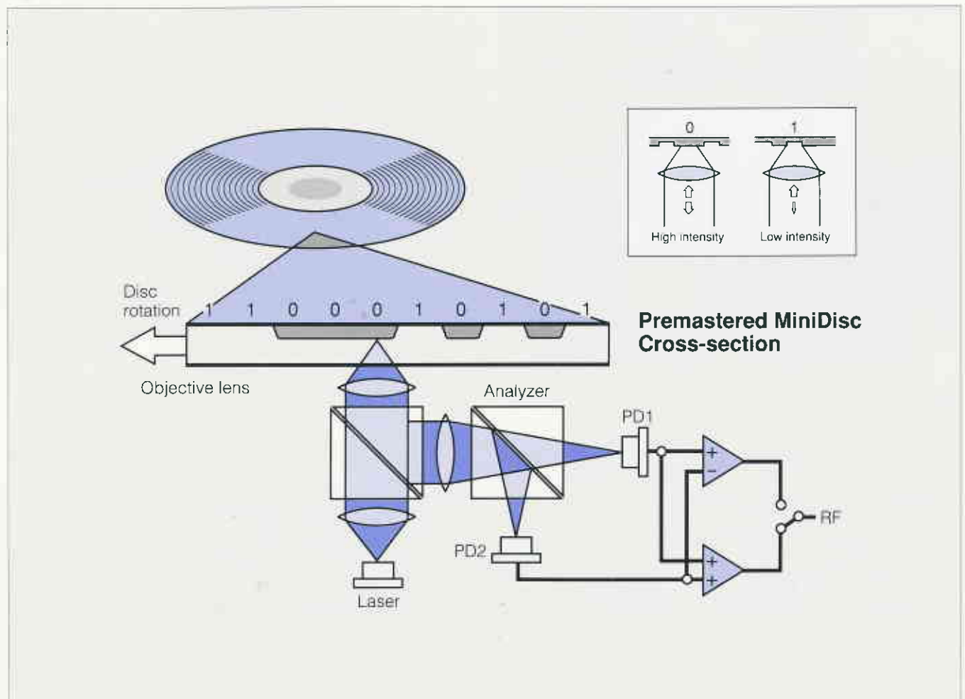
Fig. 13 Playback of Playback-only MiniDisc
