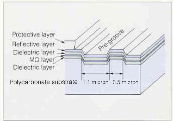
Fig. 11 MO Layered Construction of a Recordable MiniDisc
