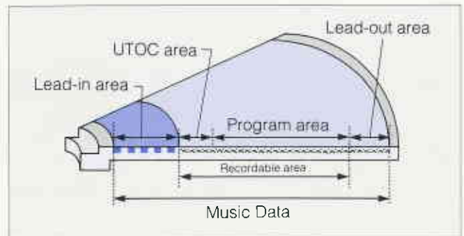
Fig. 9 Cross-section of a Recordable MiniDisc
