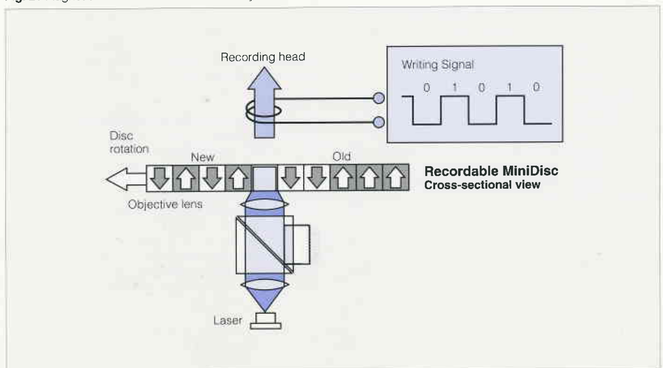
Fig. 21 Magnetic Field Modulation Overwrite System
