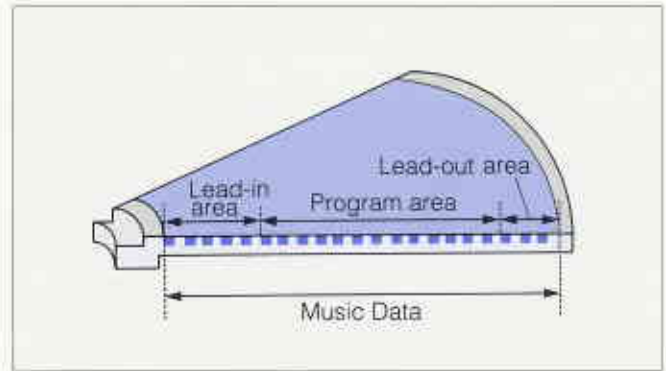
Fig. 7 Cross-section of a Playback-only MiniDisc
