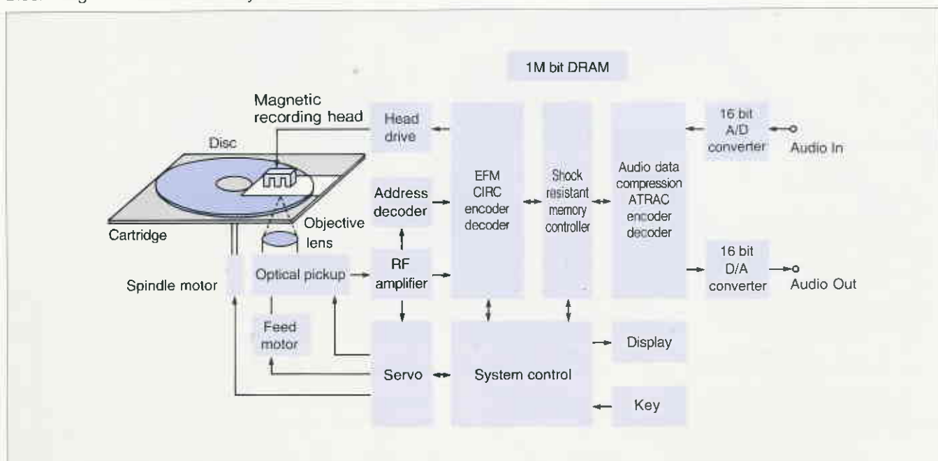
Block Diagram of the MiniDisc System
