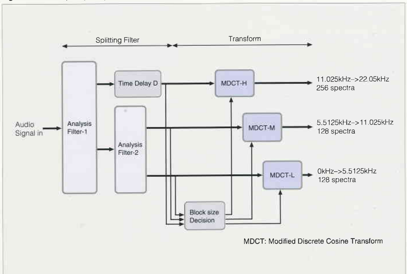
Fig. 18 ATRAC Frequency Analysis Circuit Construction
