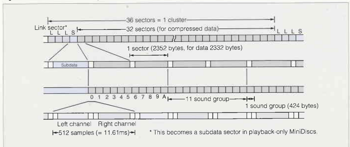
Fig. 6 MiniDisc Data Format Configuration
