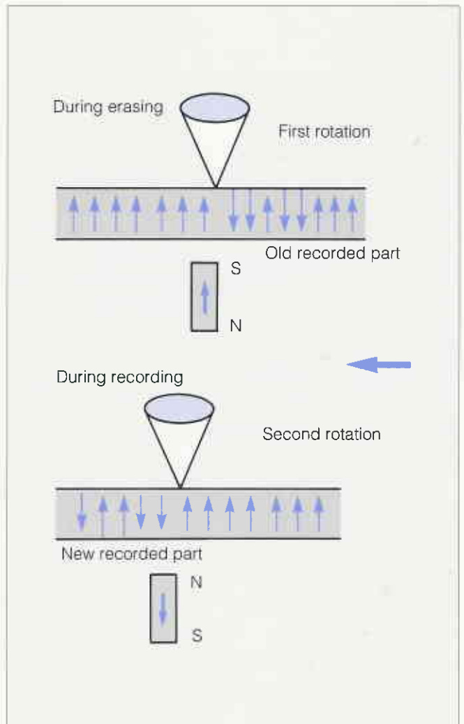
Fig. 20 Data Rewriting with One Laser in Two Rotations
