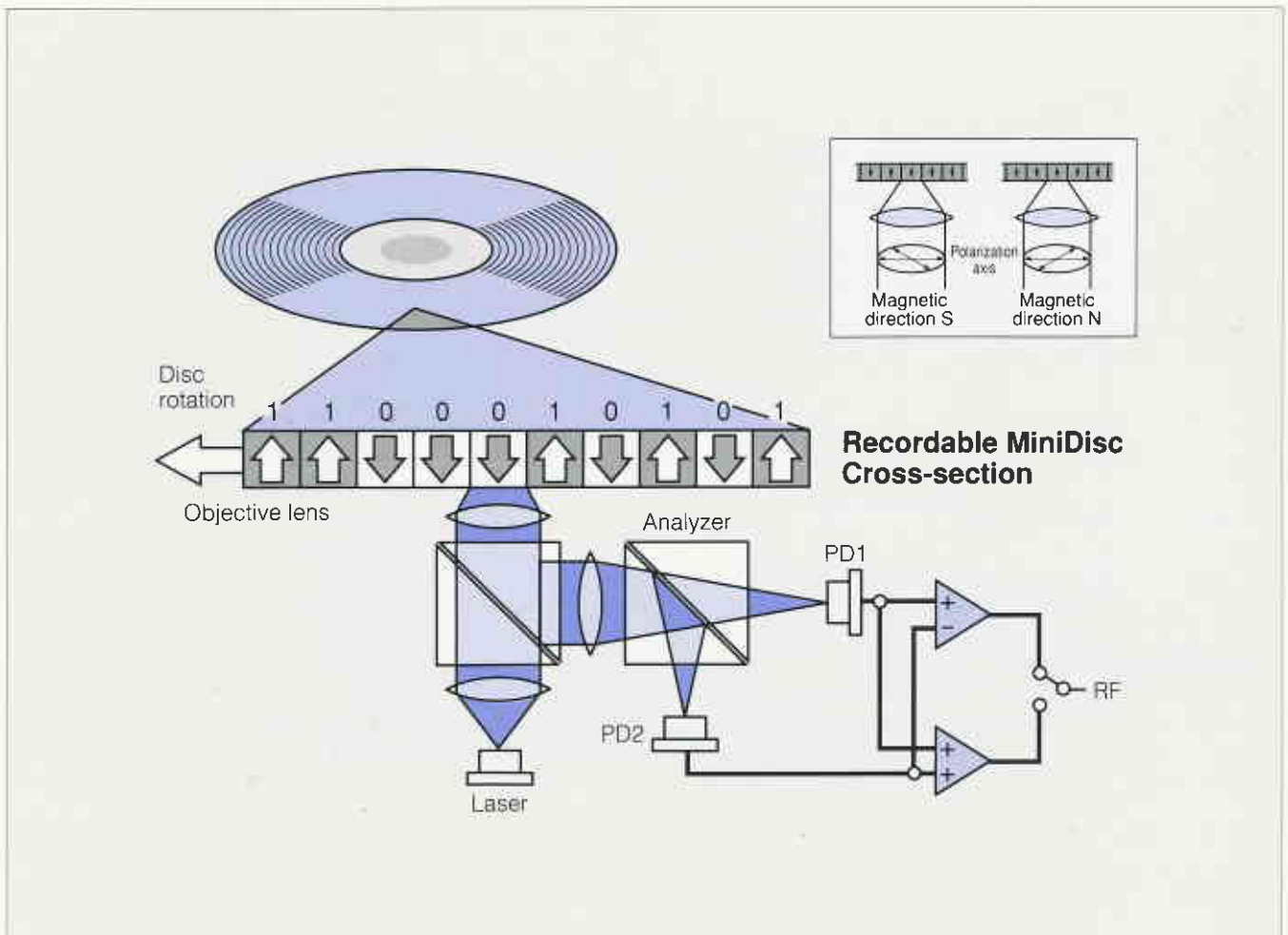
Fig. 14 Playback of a Recordable MiniDisc
