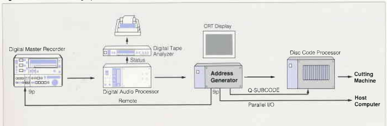
Fig. 28 MiniDisc Mastering System
