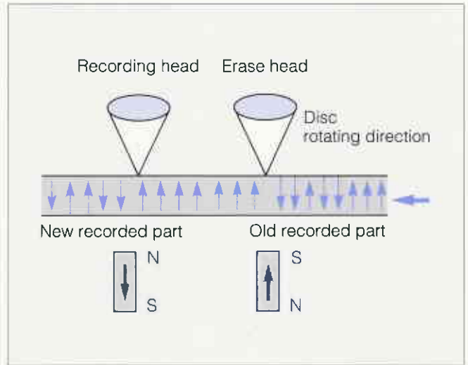
Fig. 19 Data Rewriting with Two Lasers in One Rotation
