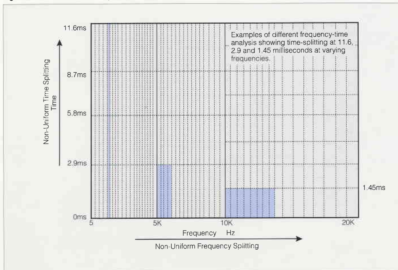
Fig. 17 ATRAC Non-Uniform Frequency-Time Splitting
