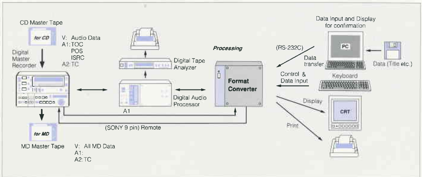
Fig. 26 MiniDisc Premastering System
