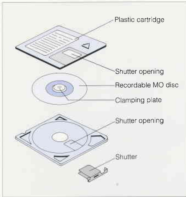
Fig. 10 Exploded View of a Recordable MiniDisc
